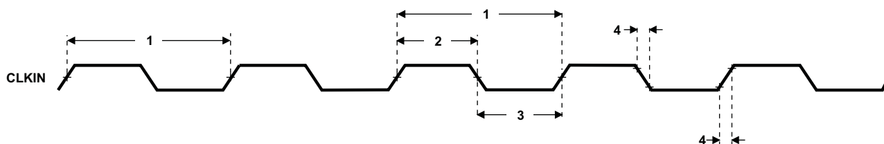
Figure 6-9. CLKIN Timing
