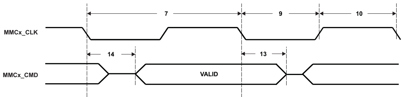
Figure 6-22. MMC/SD Host Command Write Timing
