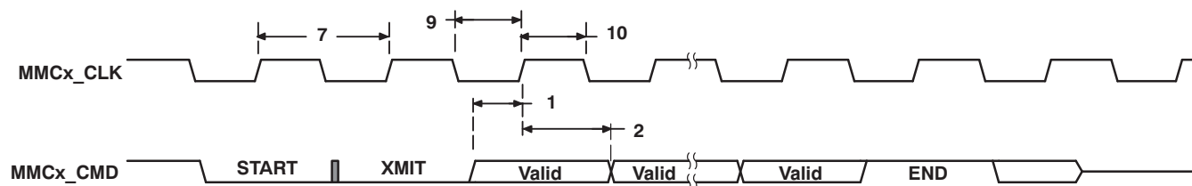
Figure 6-24. MMC/SD Host Write Timing
