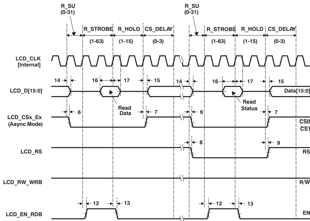
Figure 6-34. Micro-Interface Graphic Display 6800 Status
